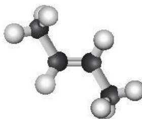
trans -but-2-ene
