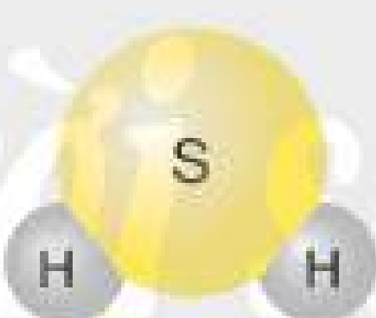
b) Hydrogen sulfide
