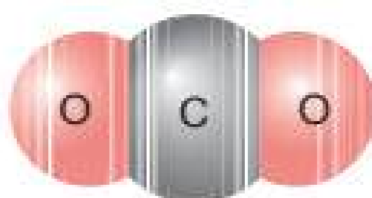
b) Carbon dioxide
